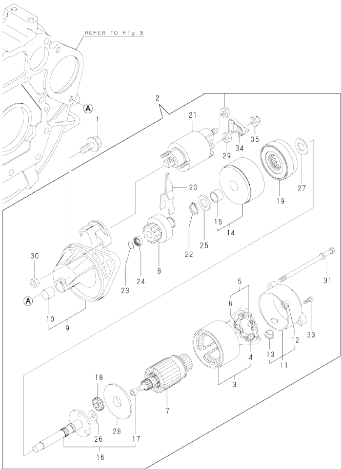
Fig.14. STARTER MOTOR
