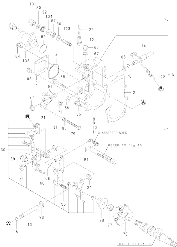
OCR10-M57900 ENGINE Fig.11. GOVERNOR
