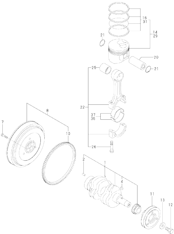
OCR10-M57900 ENGINE Fig.7. CRANKSHAFT & PISTON
